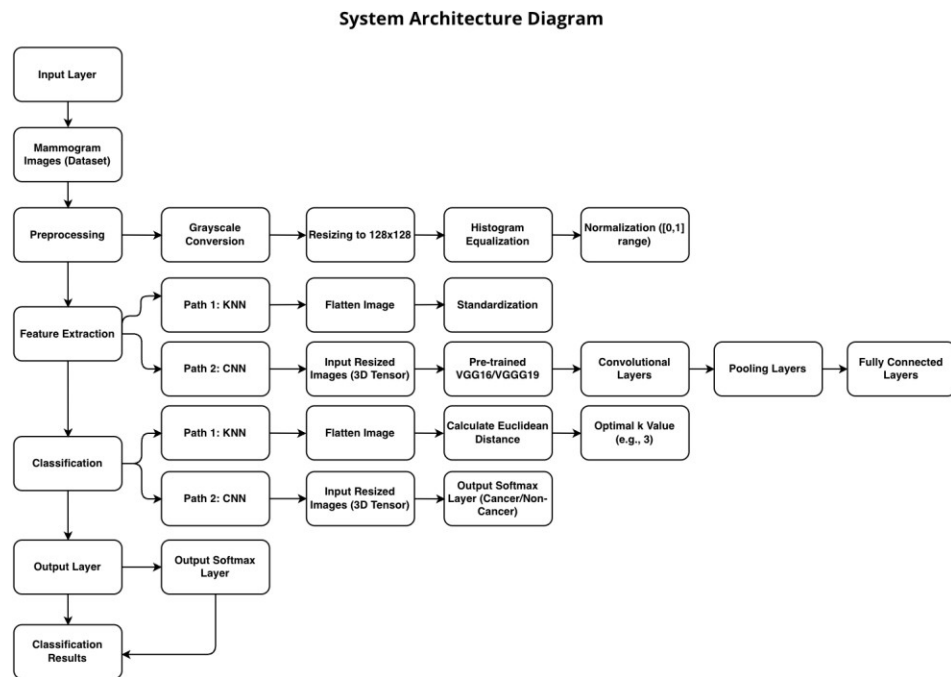
Figure 3.2 System Architecture Diagram.
