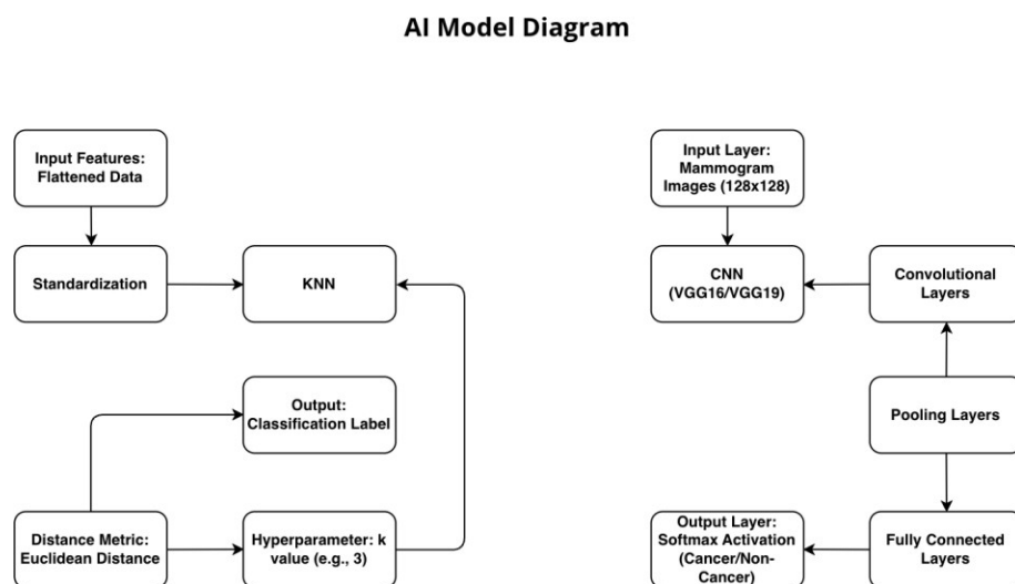
Figure 3.3 AI Model Diagram.
